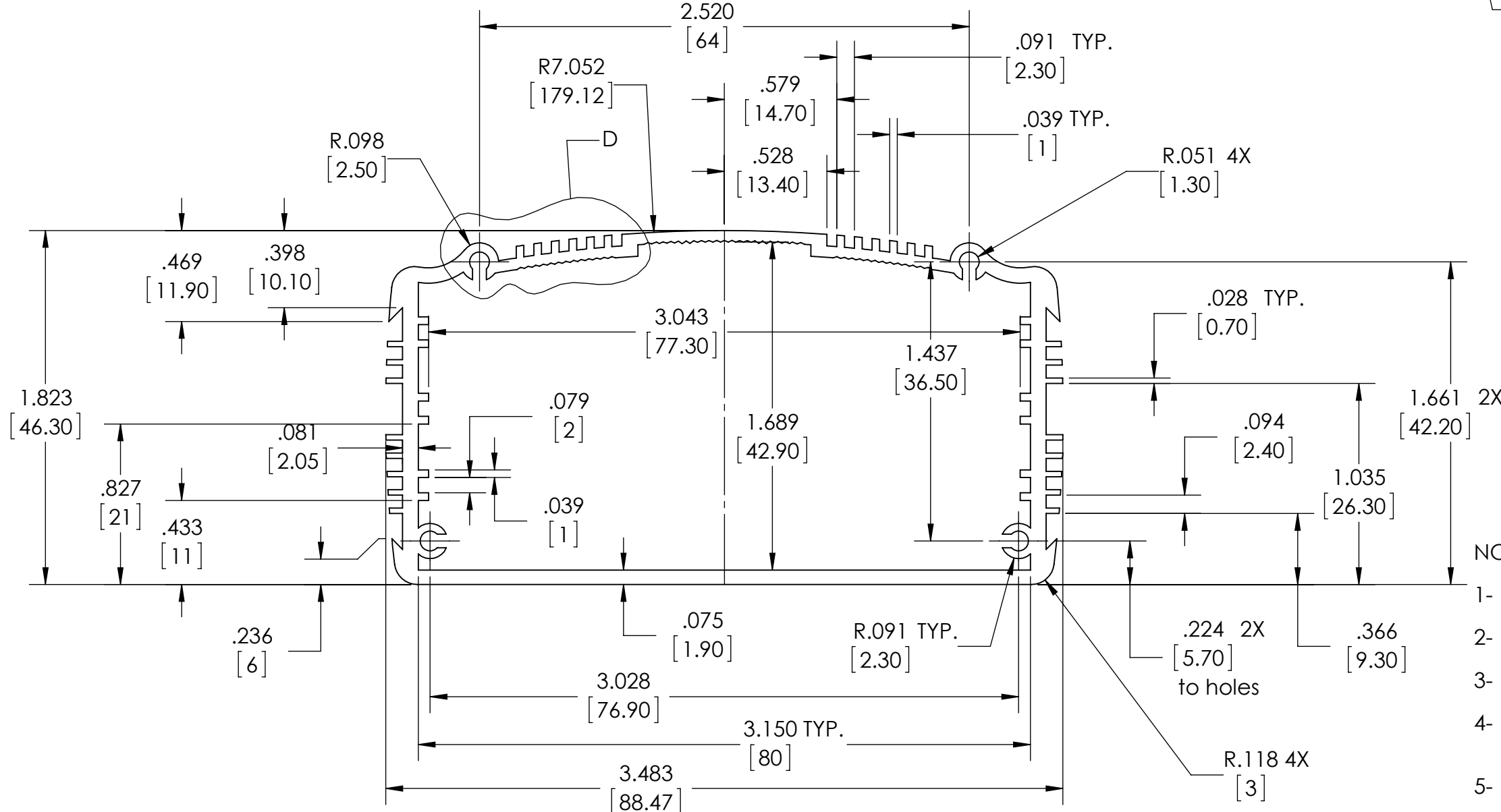
EXTRUSION PROFILE
